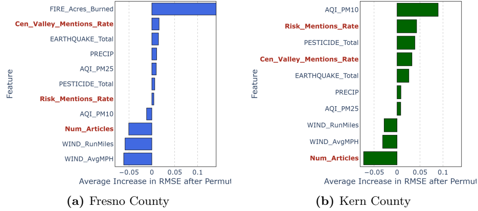
Fig. 4: Average permutation feature importance (PFI) scores across 100 LSTM runs for (a) Fresno County and (b) Kern County. Media-related variables are highlighted in red.
