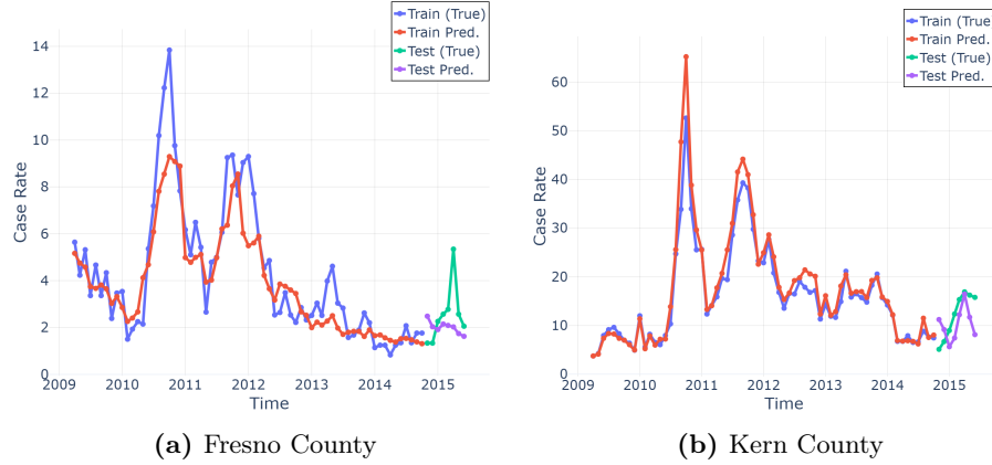
Fig. 3: LSTM model predictions and observed Valley Fever case rates across one run for (a) Fresno County and (b) Kern County.
