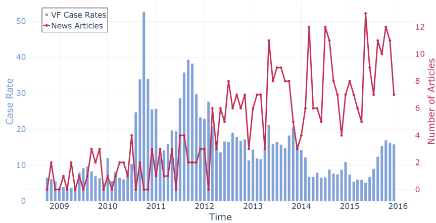
Fig. 2: Kern County monthly Valley Fever (VF) case rates and news article volume from 2008 to 2016.
