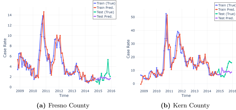
Fig. 5: SARIMAX model predictions and observed Valley Fever case rates across one run for (a) Fresno County and (b) Kern County.
